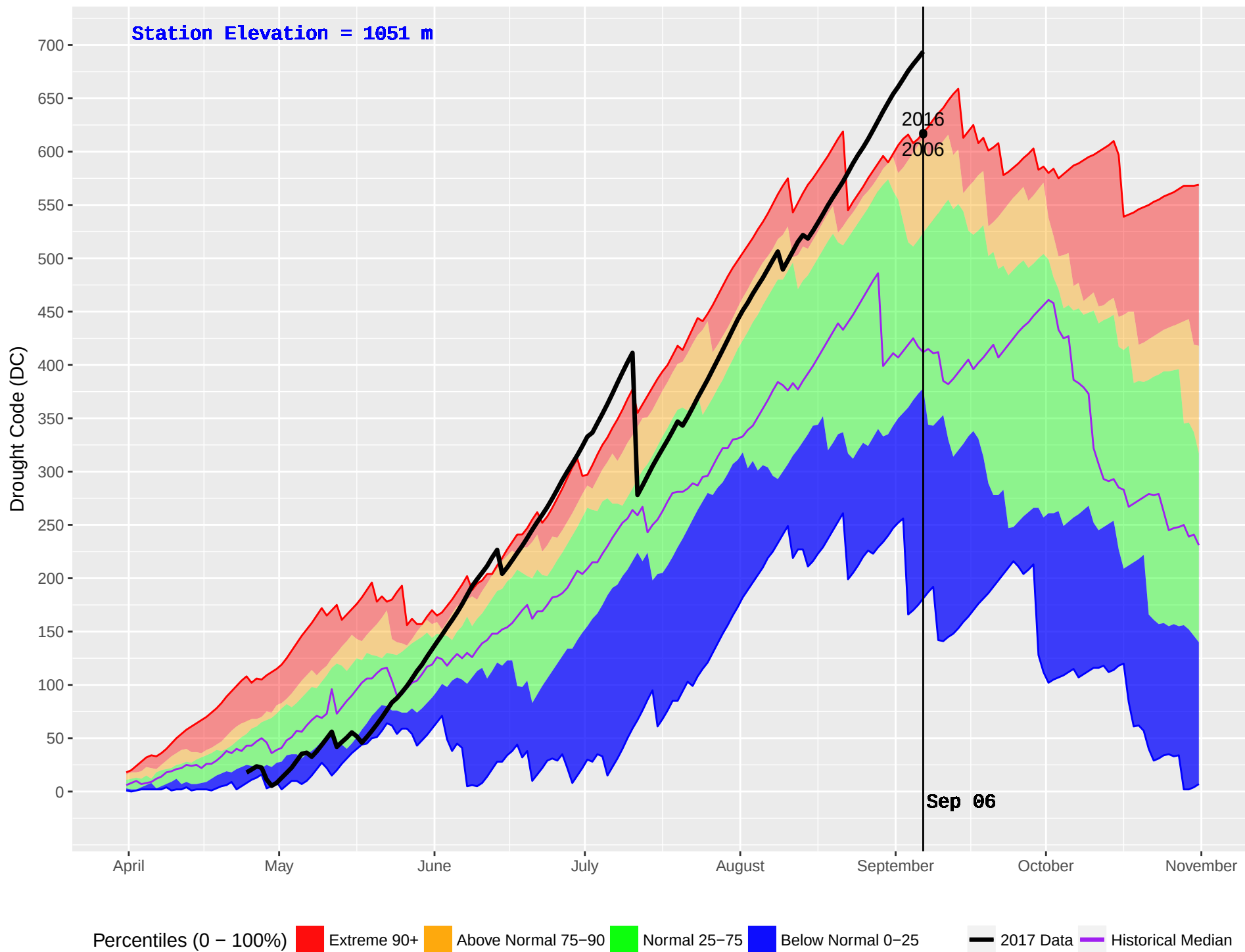
GOATHAVEN (886) : Historical (2005–2016) and Current (2017) Noon Drought Code (DC)
