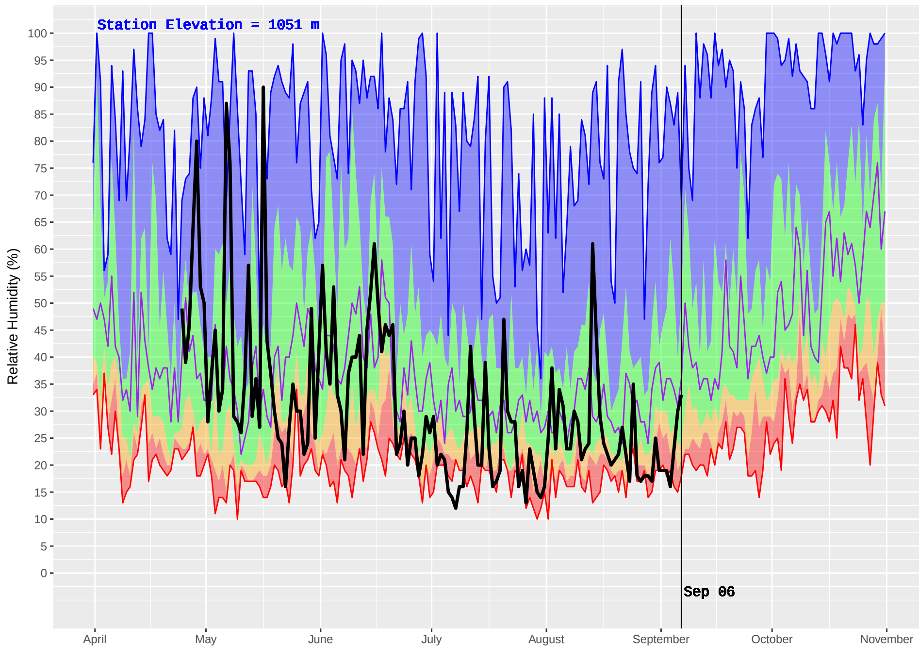
GOATHAVEN (886) : Historical (2005–2016) and Current (2017) Noon Relative Humidity
